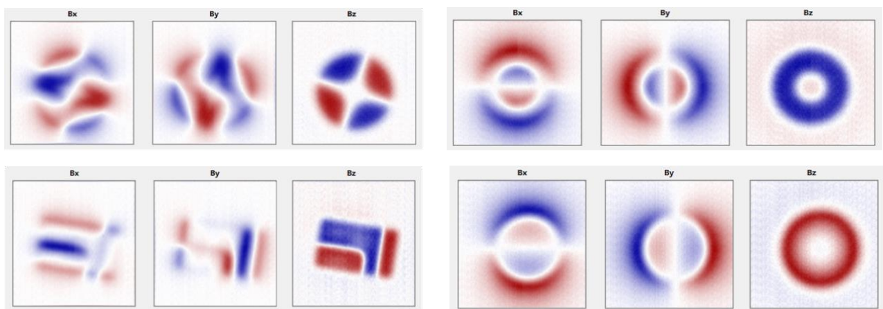
Figure 3: True 3-axis magnetic field measurements with SEN-3D-CAM-CBL
