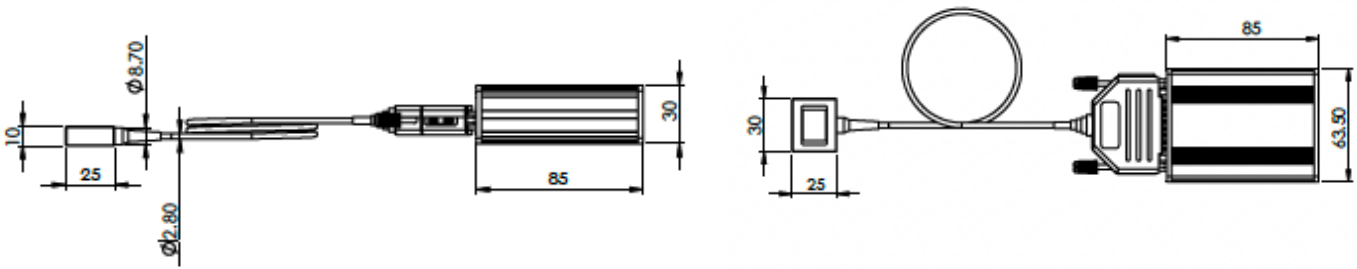
Figure 4: Structure and dimensions of the SEN-3D-CAM-CBL
